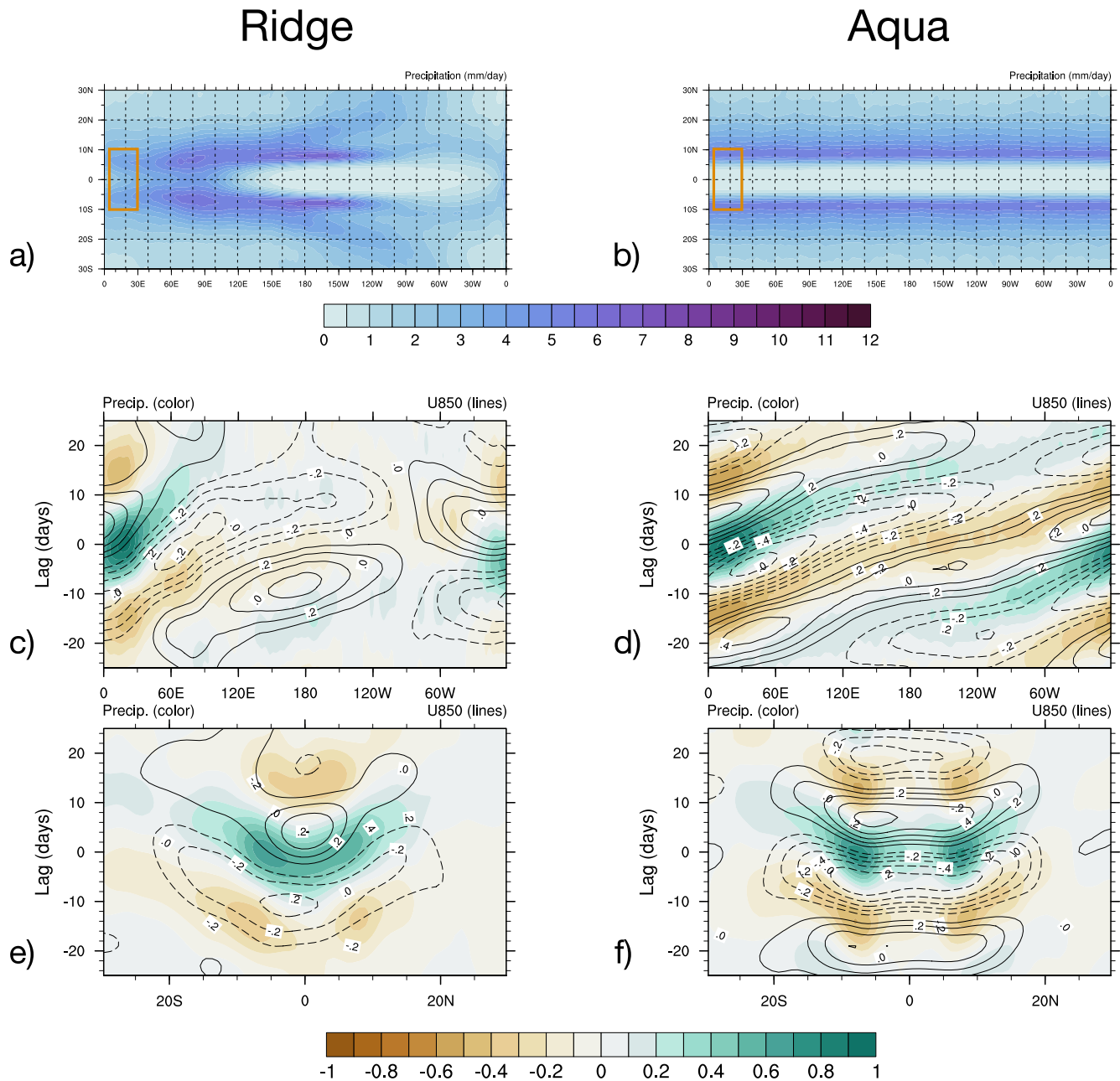
Figure 2. The propagation of the Madden-Julian Oscillation (MJO)-like mode, using data from Yr 401–420. (a and b) The climatology of annual average precipitation ( \text{mm day}^{-1} ). (c–f) Lagged correlation of the filtered signal with 20–100 day period in precipitation (colored shading) and low-level zonal wind at 850 hPa (contour line), across the zonal direction (c–d) and meridional direction (e–f). The orange box of 10^{\circ}\text{N} – 10^{\circ}\text{S} , 5^{\circ} – 30^{\circ}\text{E} in panels (a and b) marks the reference location of the lagged correlation in panels (c–f).
