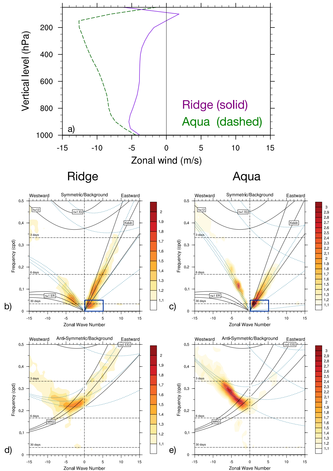
Figure 1. The interaction between the zonal mean flow and convectively coupled equatorial waves, using data from Yr 401–420. (a) Vertical profiles of the zonal mean zonal wind, averaged between 15°N and 15°S. (b–e) Wheeler-Kiladis diagrams of 6-hourly precipitation, averaged between 15°N and 15°S. The solid black curves represent the theoretical dispersion relations assuming zero zonal flow, whereas the dashed blue curves represent the dispersion relations Doppler-shifted by the background zonal flow of -5 \text{ m s}^{-1} for Ridge (b and d), and -10 \text{ m s}^{-1} for Aqua (c and e).
