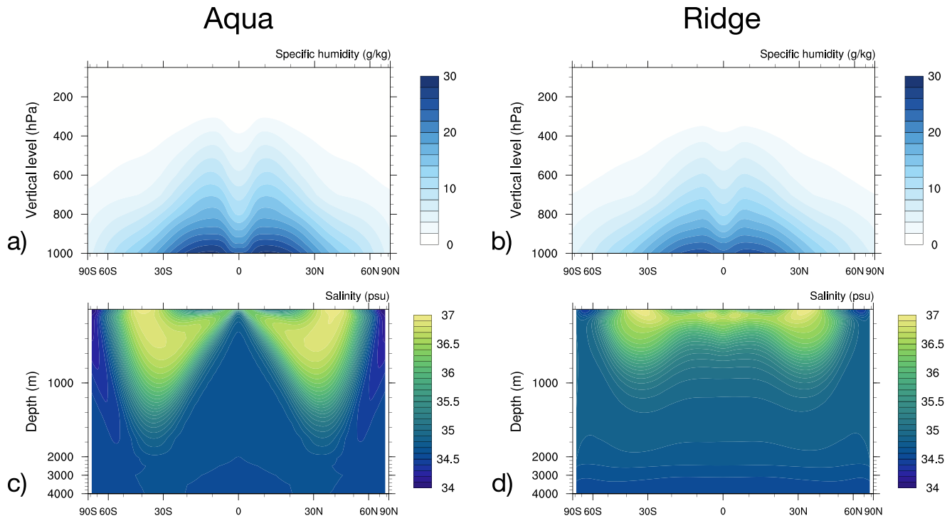
Figure 5. Zonally averaged vertical sections, 100-years climatology. (a–b) Specific humidity ( \text{g kg}^{-1} ). (c–d) Salinity (psu). For the ocean (c–d), the depths below 2,000 m are linearly shrunk as labeled.
