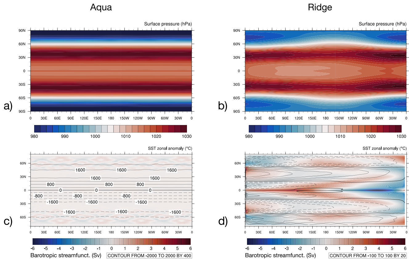
Figure 6. Plan views of 100-year climatology. (a–b) Atmosphere: surface pressure (hPa). (c–d) Ocean: barotropic streamfunction (Sv, contour lines; solid is positive/clockwise, dashed is negative/counterclockwise), overlaid on the zonal anomaly of SST (°C, color shading). Note the difference in contouring intervals for the streamfunction (c–d). The pattern of Aqua’s SST zonal anomaly (panel c), barely visible, reflects the imprints of bottom topography.
