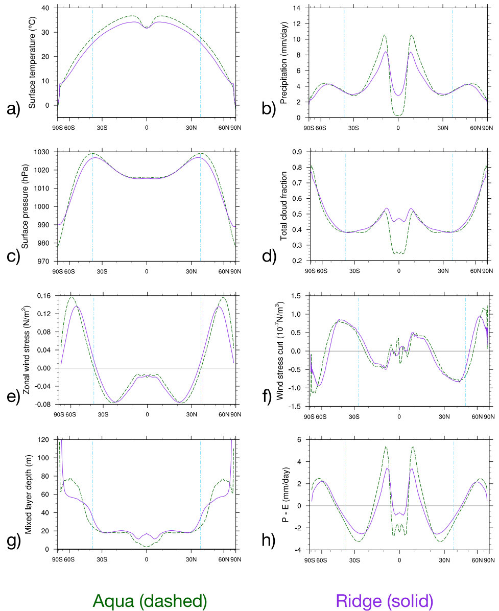
Figure 4. Zonal average profiles, 100-years climatology. (a) Surface temperature ( ^{\circ}\text{C} ). (b) Precipitation rate ( \text{mm day}^{-1} ). (c) Surface pressure (hPa). (d) Total cloud fraction. (e) Zonal wind stress ( \text{N m}^{-2} ). (f) Curl of zonal wind stress ( 10^{-7} \text{ N m}^{-3} ). (g) Ocean mixed layer depth (m). (h) Precipitation minus evaporation ( \text{mm day}^{-1} ). The vertical blue lines mark the extent of the tropics, as defined by TOA radiative budget (see Figure 3).
