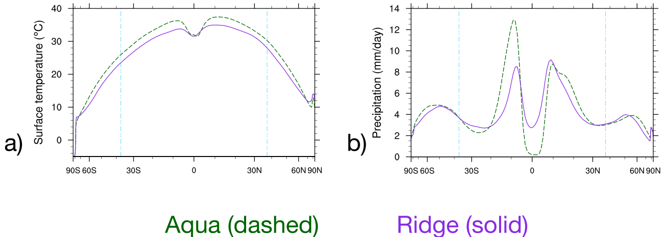
Figure 10. As Figures 4a and 4b, but for boreal summer (June, July, and August).
