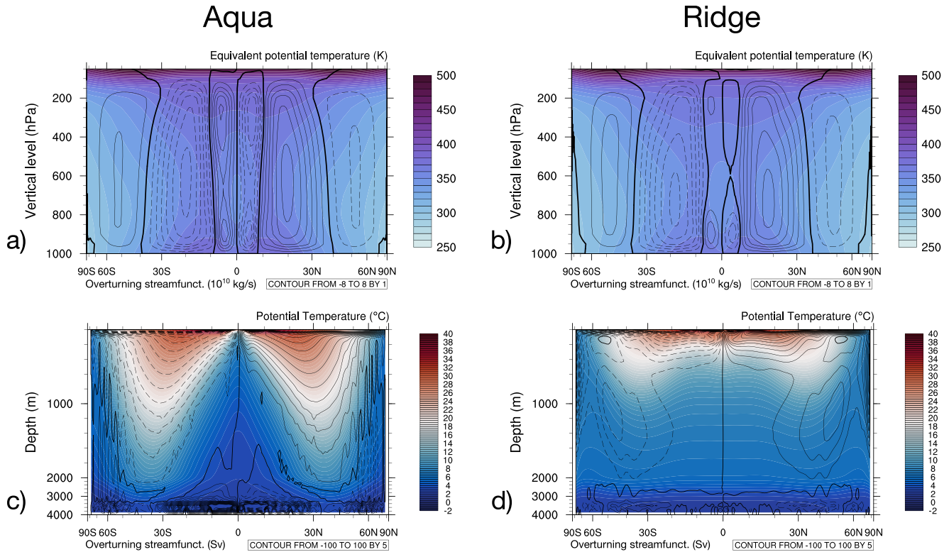
Figure 8. Zonally averaged vertical sections, 100-years climatology. (a–b) Atmosphere: Eulerian meridional overturning streamfunction ( 10^{10} \text{ kg s}^{-1} , contour lines; solid is positive/clockwise, dashed is negative/counterclockwise), overlaid on equivalent potential temperature (K, colored shading). (c–d) Ocean: residual overturning streamfunction (Sv, contour lines; solid is positive/clockwise, dashed is negative/counterclockwise), overlaid on potential temperature ( ^{\circ}\text{C} , colored shading). The overturning cells in the ocean are closed to within the magnitude of atmospheric moisture transport in the surface mixed layer (see P–E in Figure 4h).
