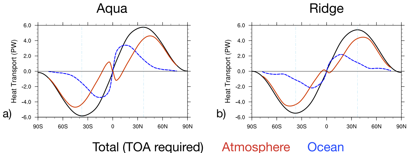
Figure 12. Meridional heat transport, 100-years climatology. (a) Aqua. (b) Ridge. The vertical blue lines mark the extent of the tropics, as in Figures 3a–3d and Figure 4.
