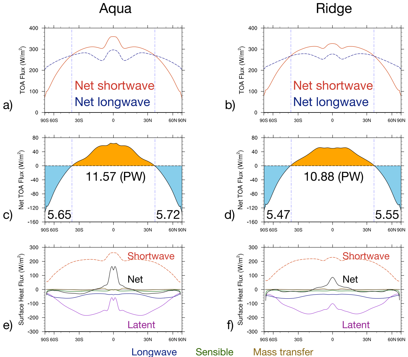
Figure 3. Zonally averaged energy budgets, 100-years climatology. (a–b) Top-of-atmosphere (TOA) fluxes ( \text{W m}^{-2} ). (c–d) Net TOA flux ( \text{W m}^{-2} ) derived from (a–b), labeled with the integrated total amount of tropical surplus (shaded in orange) and extratropical deficit (shaded in blue), in petawatt (PW). (e–f) Ocean surface heat fluxes ( \text{W m}^{-2} ). The x -axis is scaled by \sin(\text{lat}) to reflect the proportion of surface area, with minor tick marks at 10^\circ intervals.
