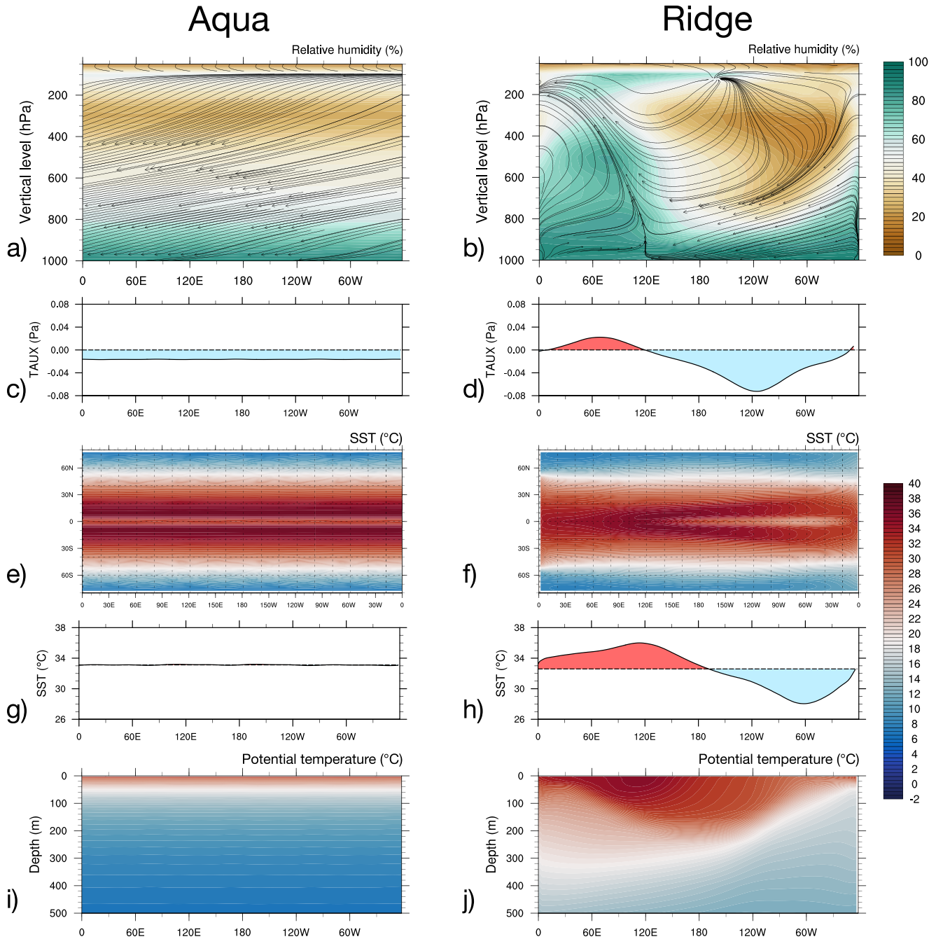
Figure 2. Zonal features in the tropics, 100-years climatology. (a–b) Zonal circulation in the atmosphere with Walker-like feature on Ridge, seen in relative humidity (colored shading), and streamline of zonal and vertical velocity (solid arrows). Vertical velocity is scaled by a factor of 50 for visualization. (c–d) Zonal gradient of zonal wind stress (Pa), the dashed horizontal line marking 0; (e–f) SST (°C). (g–h) Zonal gradient of SST (°C), the dashed horizontal line marking the zonal average value. (i–j) Equatorial thermocline, as seen in potential temperature (°C). All panels except for (e–f) are averaged 5°N–5°S.
