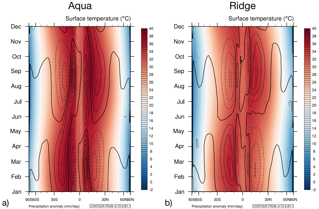
Figure 9. The seasonal cycle of zonally averaged surface temperature ( ^{\circ}\text{C} , colored shading) and precipitation anomaly from the annual mean ( \text{mm day}^{-1} , contour lines; solid is positive, dashed is negative), 100-years climatology. (a) Aqua. (b) Ridge.
