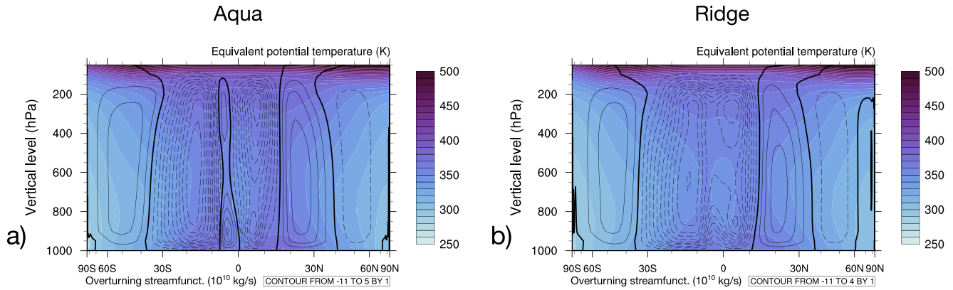
Figure 11. As Figures 8a and 8b, but for boreal summer (June, July, and August).
