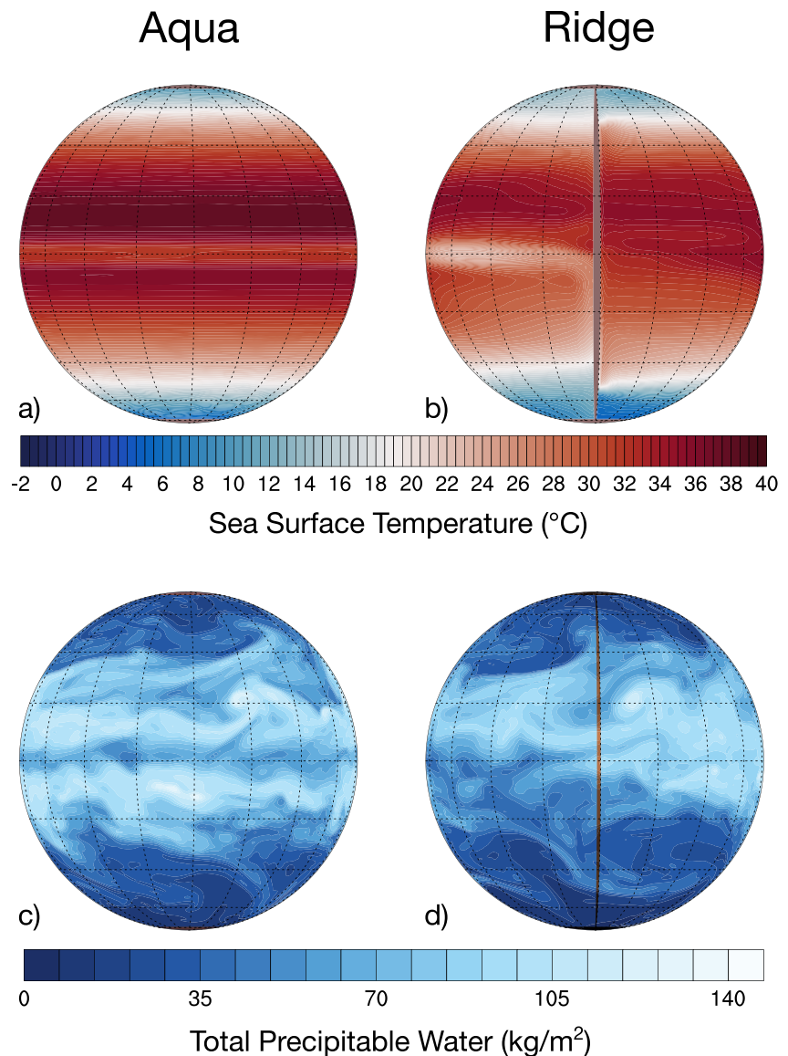
Figure 1. Illustration of the Aqua and Ridge planets. The polar land caps and the ridge continent are marked in brown. (a–b) SST (°C) for August (100-years climatology), showing the global cold belt of equatorial upwelling on Aqua, and the eastern and western boundary currents on Ridge (see animation of the seasonal cycle in supplement). (c–d) Instantaneous snapshots of total precipitable water ( \text{kg m}^{-2} ) from boreal summer, displaying various synoptic systems.
