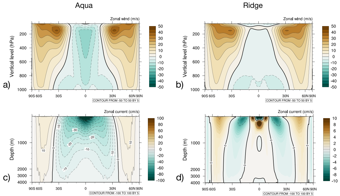
Figure 7. Zonally averaged vertical sections, 100-years climatology. (a–b) Atmosphere: zonal wind ( \text{m s}^{-1} ). (c–d) Ocean: zonal current ( \text{cm s}^{-1} ). The color scale of panel (c) is an order of magnitude greater than panel (d).
