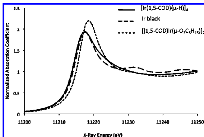
Figure 3. XANES of the [\text{Ir}(1,5\text{-COD})(\mu\text{-H})_4] complex and reference compounds used of formally \text{Ir}^0 black and formally \text{Ir}^I in [(1,5\text{-COD})\text{Ir}(\mu\text{-O}_2\text{C}_8\text{H}_{15})_2] . 11
