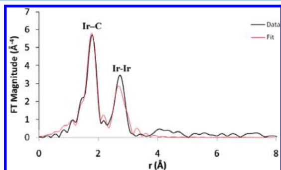
Figure 2. FT magnitudes of Ir L_3 -edge EXAFS data for the [(1,5\text{-COD})\text{Ir}(\mu\text{-H})_4] complex (black) and its associated fit using Ir–C and Ir–Ir contributions (red).
