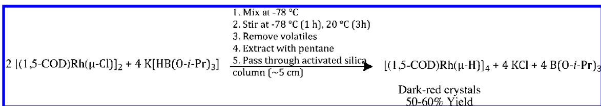
Scheme 1. Balanced Reaction Stoichiometry and the Reaction Conditions for the Synthesis of [\text{Rh}(1,5\text{-COD})(\mu\text{-H})]_4 (Adapted from Reference 3a)
