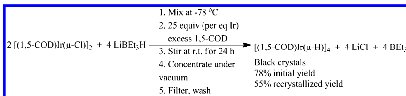
Scheme 2. Balanced Reaction Stoichiometry and Reaction Conditions of the Successful Synthesis of [\text{Ir}(\text{1,5-COD})(\mu\text{-H})]_4
