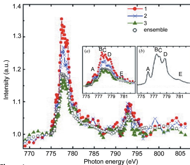
Figure 1 X-ray absorption spectra at the Co L_{2,3} -edges as a function of the incident X-ray energy of three different cobalt particles of \sim 8 nm in diameter. The insets compare (a) the L_3 peak region of the particles with (b) the L_3 -edge peak region of a reference CoO film. The spectrum with open circles in (a) represents the average of the X-ray absorption spectra of 23 different nanoparticles. [From J. Magn. Magn. Mater. 326 , 426–428, Rodríguez et al. (2007). Copyright (2007), with permission from Elsevier.]
