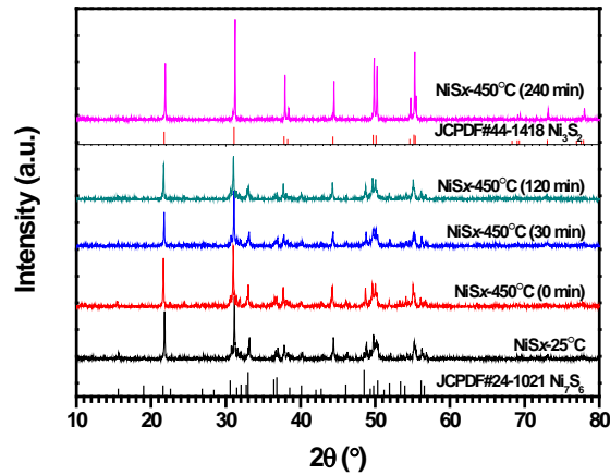
Figure 1. XRD patterns of NiS_x measured at room temperature after reduction at different temperatures and durations.
