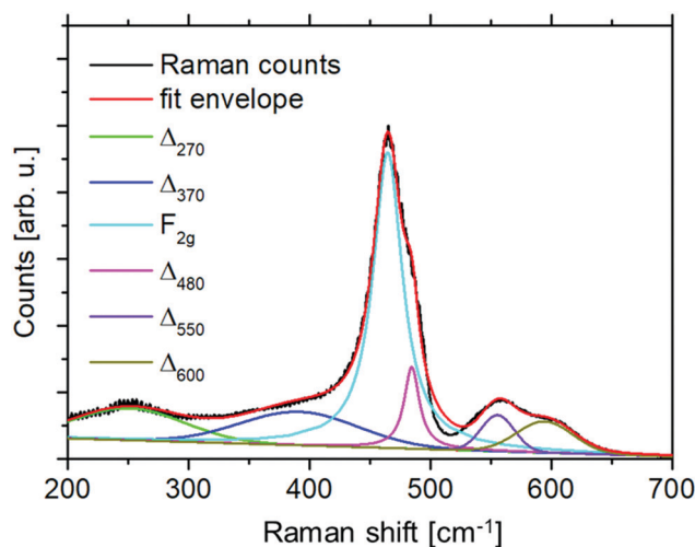
Fig. 28 Raman spectrum of a high temperature sintered Ce 0.8 Gd 0.2 O 1.9 pellet, with peak fit for the F_{2g} vibrational mode and various defect-related Raman peaks, labeled with \Delta . Experimental details are in the ESI, † Section S2 measured by Rupp group on polycrystalline pellets.
