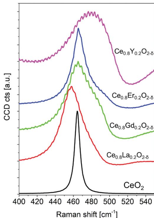
Fig. 26 Raman spectra around the F_{2g} peak in ceria pellets doped with 20 mol% La, Gd, Er, and Y, normalised to the F_{2g} peak height established by Rupp group, see ESI, † Section S2 for experimental details.
