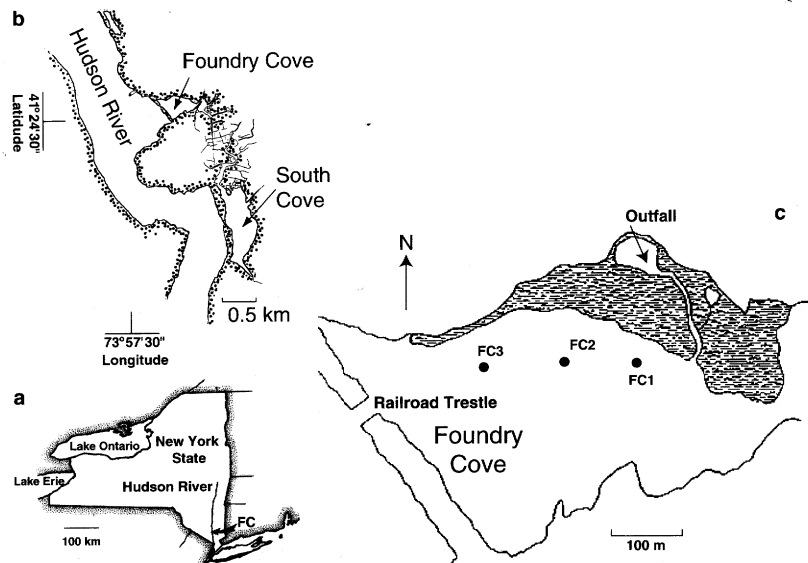
Fig. 1. Maps indicating geographic location of study sites (Foundry and South Coves) (a & b) and locations within Foundry Cove (FC 1, FC 2 and FC 3) where sediment and oligochaetes were collected for use in Cd accumulation and trophic transfer studies (c). Site of the former battery plant outfall is also indicated
