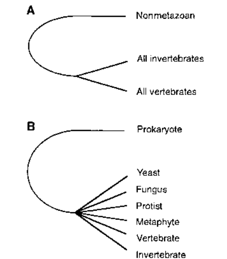
Fig. 3. Relative rate tests. Diagrams illustrate the scheme used to test for homogeneity of sequence divergence rates among metazoan phyla (A) and among eukaryotic kingdoms (B). The test results (Tables 3 and 4) indicate similar branch lengths and therefore similar rates of sequence divergence in both cases.
