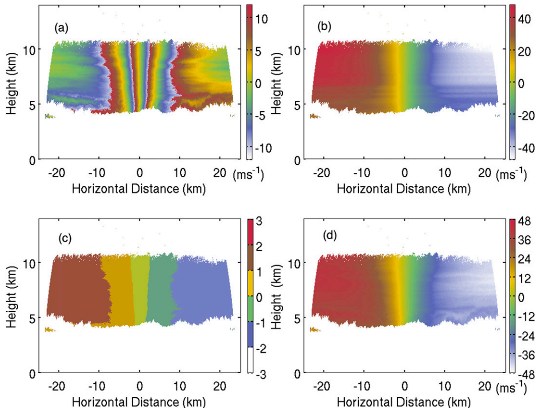
FIG. 7. (a) Ka-SACR Doppler velocity field during a horizon-to-horizon RHI scan, (b) the first-guess Ka-SACR Doppler velocity field, (c) the number of foldings, and (d) the unfolded Doppler velocity field.
