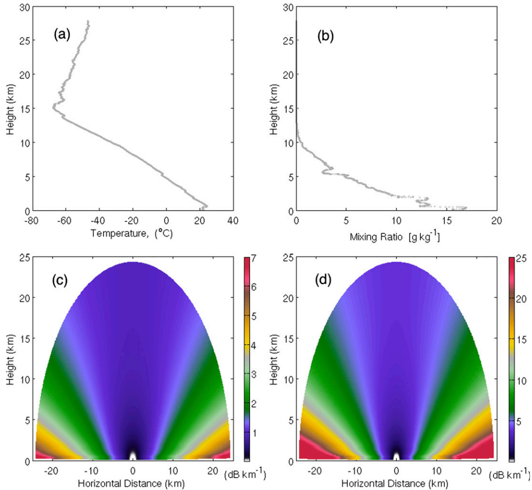
FIG. 4. (a) Temperature and (b) mixing ratio profiles from a sounding launched on 27 Jul 2012, during the ARM Mobile Facility deployment in Cape Cod; estimated two-way gaseous attenuation as a function of elevation angle and range for (c) Ka-SACR and (d) W-SACR.
