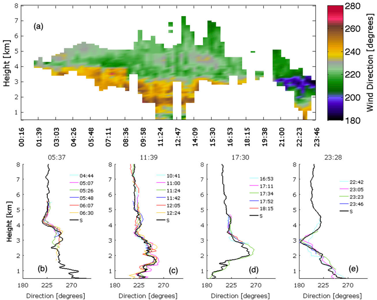
FIG. 11. (a) Diurnal evolution of the retrieved wind direction at heights where cloud and/or precipitation was detected by the SWACR on 1 May 2010; (b)–(e) wind direction profiles from the four SGP soundings (black lines) and wind direction profiles retrieved by the VAD technique applied to the HS-RHI scan measurements within a 3-h window centered on the sounding times (color lines). The time (UTC) of each sounding is indicated at the top of each plot, and the times of each HS-RHI set of scans used in a retrieval are indicated by the color lines with time labels in the legends.
