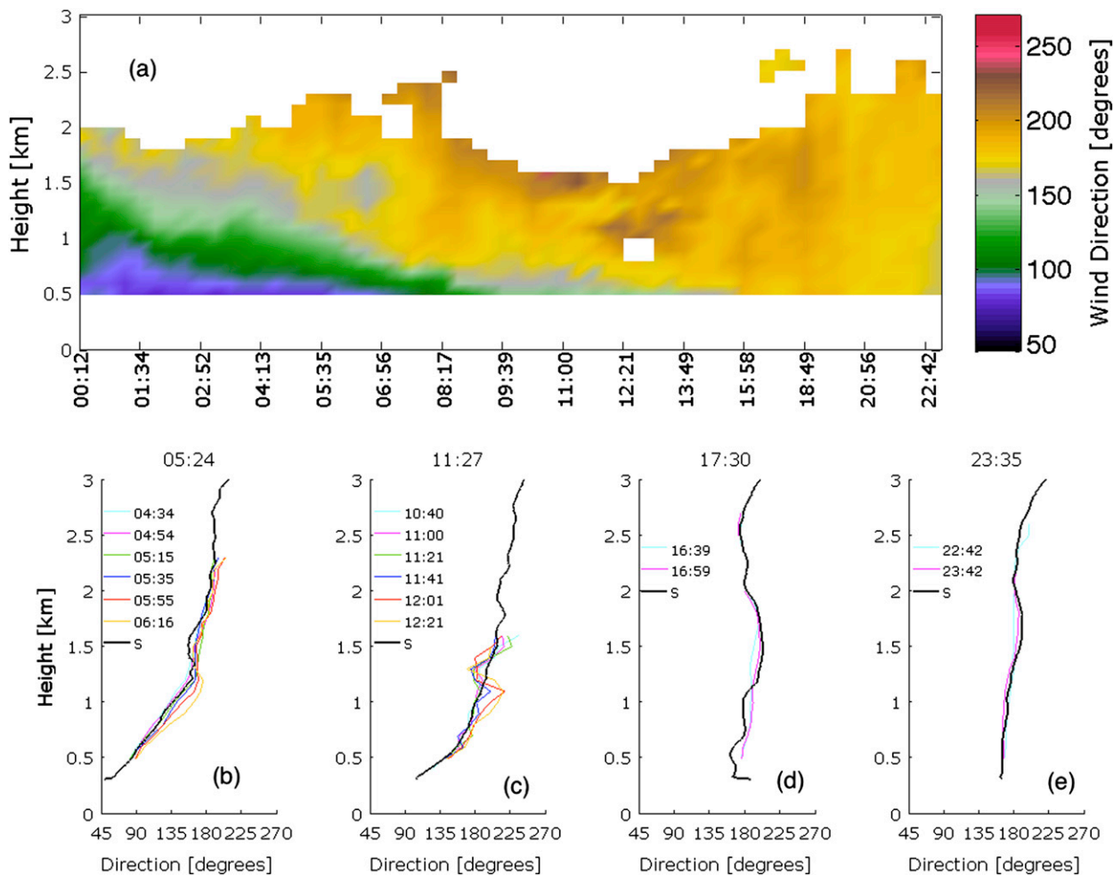
FIG. 13. (a) Diurnal evolution of the retrieved wind direction in heights where insects were detected by the SACR on 1 Jun 2011. (b)–(e) Wind direction profile from the four SGP soundings (black lines) and wind direction profile retrieved by the HS-RHI within a 3-h window around the sounding time (color lines). The time of the sounding is indicated in the title of each plot, and the HS-RHI time is also labeled on each plot.
