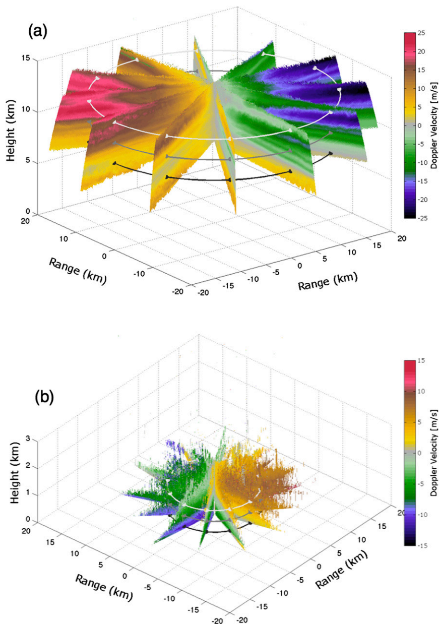
FIG. 9. Example observations of unfolded Ka-SACR mean Doppler velocities obtained from two sets of HS-RHI scans—one occurring when (a) cirrus clouds were present and the other during a period when (b) insects dominated the returns in the boundary layer.
